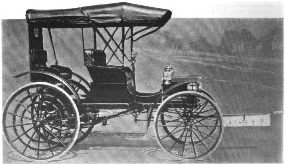
Duryea Car Rigged with a Spring Balance to Measure the Pull Required to Move It.
